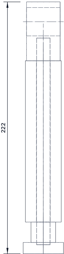
FRONT VIEW Scale 1:2; looking at the front (along +Y)
