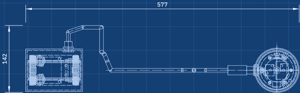
TOP VIEW Scale 1:5; looking down (along -Z)
