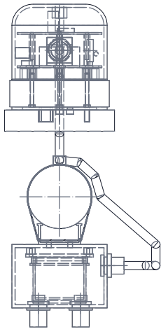
RIGHT VIEW Scale 1:5; looking at the right side (along -X)
