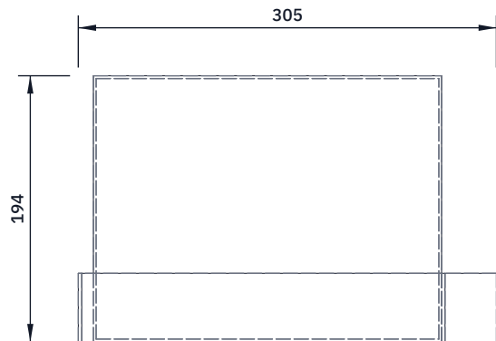
TOP VIEW Scale 1:5; looking down (along -Z)
