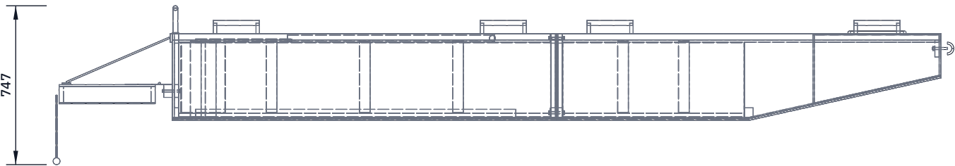
FRONT VIEW
