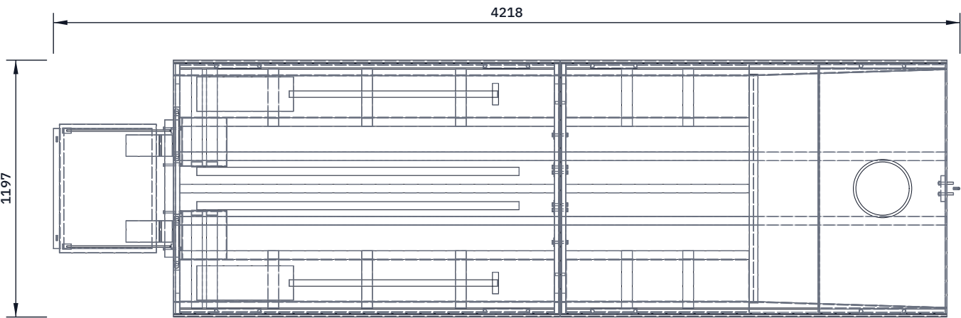
TOP VIEW
