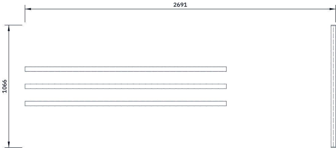
TOP VIEW Scale 1:20; looking down (along -Z)
