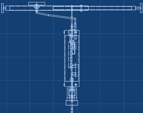
RIGHT VIEW
