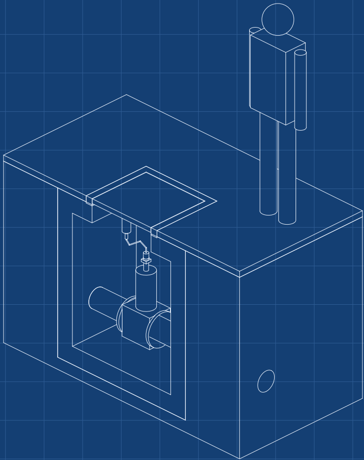
ISOMETRIC VIEW Not to scale; grey is for scale
