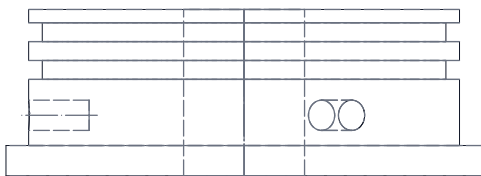
RIGHT VIEW Scale 1:1; looking at the right side (along -X)
