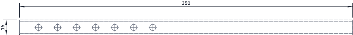
TOP VIEW
