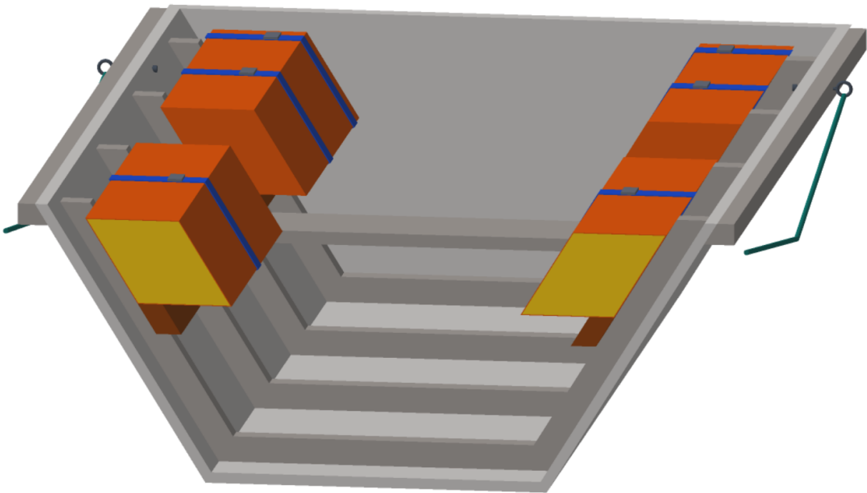
Cut across the canoe 2.25 m forward of the transom, through module 2 on each side; seen from forward and slightly to port, 12 deg elevation. The modules sit high under the gunwale, so when the canoe is swamped they cut the waterline and hold it upright
