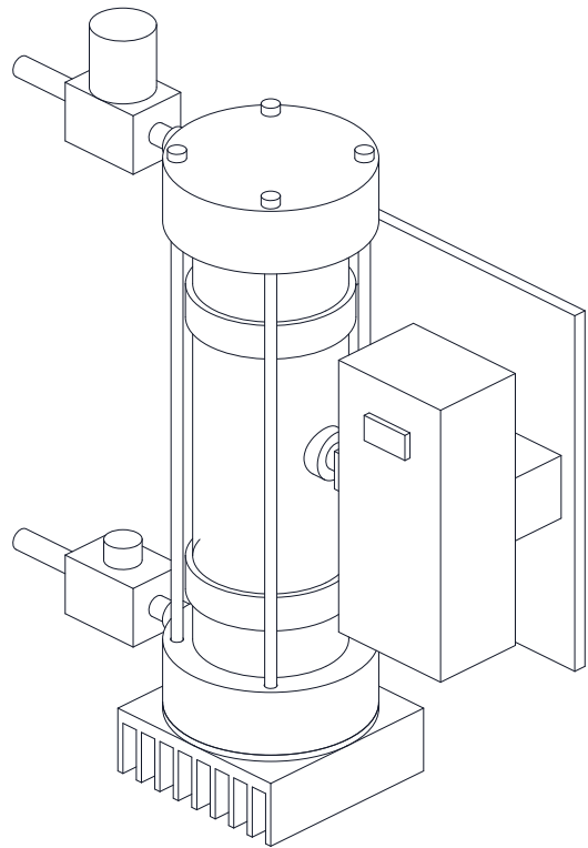
ISOMETRIC VIEW Not to scale; adapter not shown
