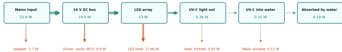
Figure 4. Power flow while water runs at 1.2 L/min. All values are estimates from LMF-CAL-001, in watts.
