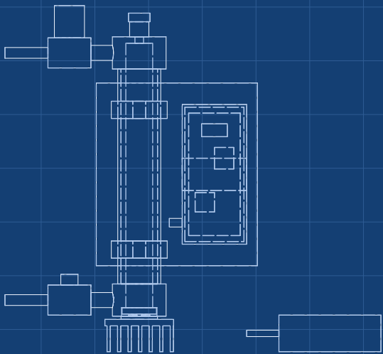
FRONT VIEW Scale 1:5
