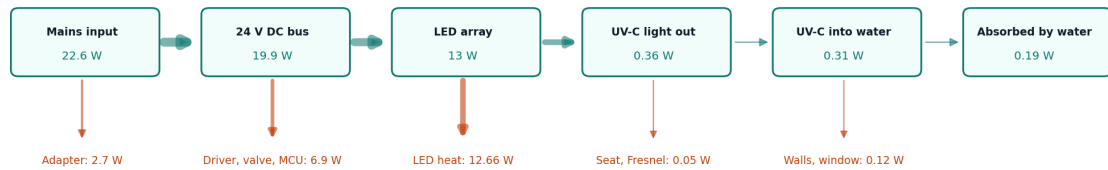
Figure 4. Power flow while water runs at 1.2 L/min. All values are estimates from LMF-CAL-001, in watts.
