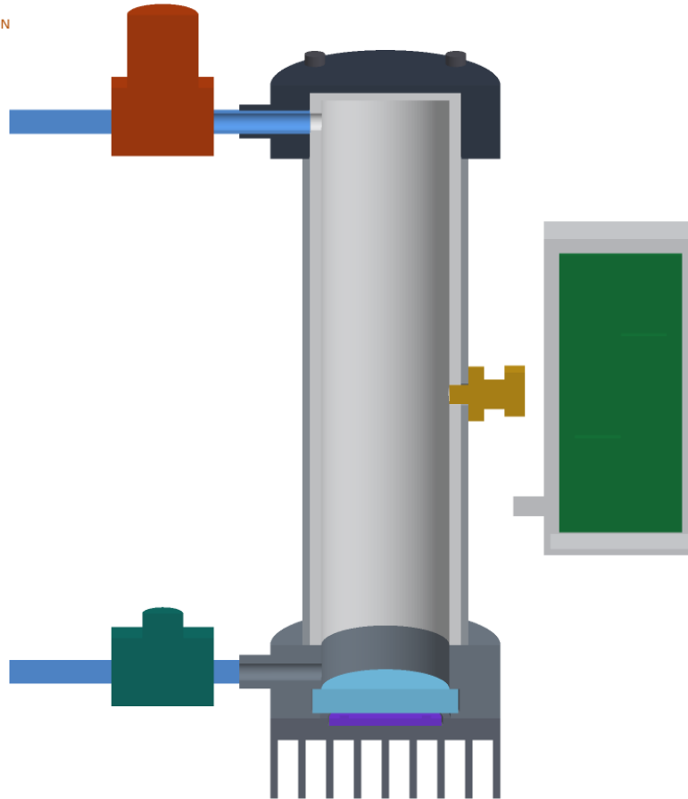
Figure 2. Cutaway through the reactor axis, looking at the wall. From the bottom: heat sink, LED board, quartz window in the stainless lower cap with the inlet, the 50 mm PTFE-lined tube with the wall photodiode on the right, and the PTFE top disc in the acetal upper cap with the outlet insert. The controller board is in the enclosure on the right.
