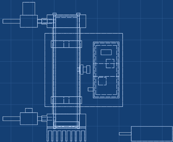
FRONT VIEW Scale 1:5
