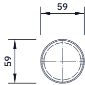
TOP VIEW Scale 1:5; looking down (along -Z)
