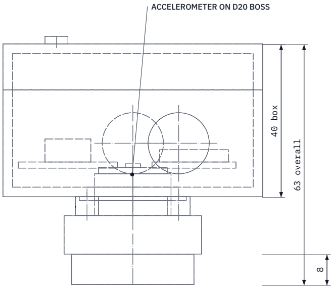
RIGHT VIEW
