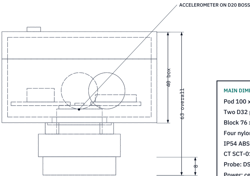
RIGHT VIEW
