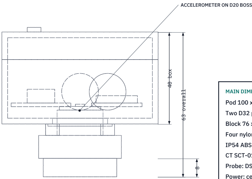
RIGHT VIEW
