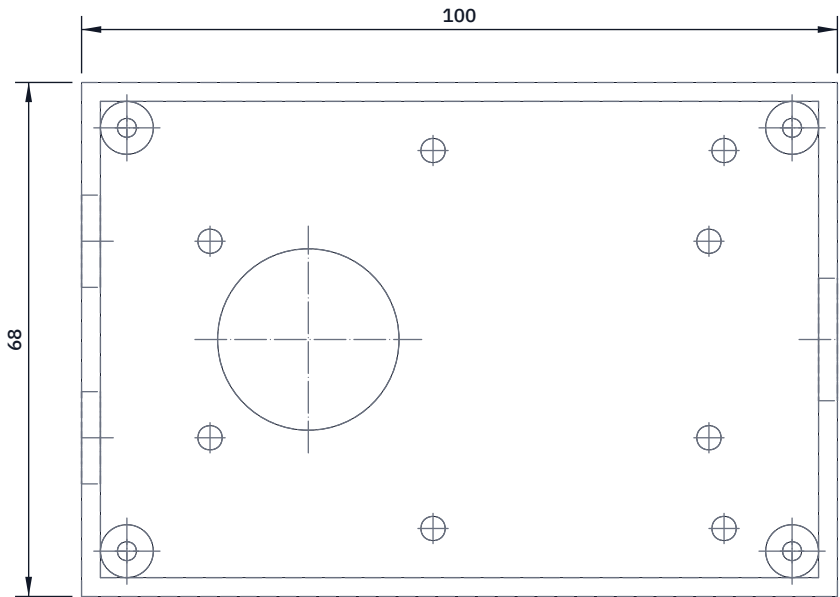
TOP VIEW Scale 1:1; looking down (along -Z)
