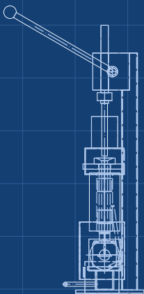
RIGHT VIEW Scale 1:20; looking at the right side (along -X)
