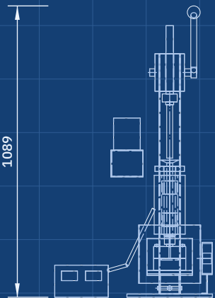
FRONT VIEW Scale 1:20; looking at the front (along +Y)
