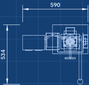
TOP VIEW Scale 1:20; looking down (along -Z)
