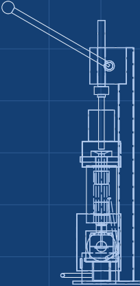
RIGHT VIEW Scale 1:20
