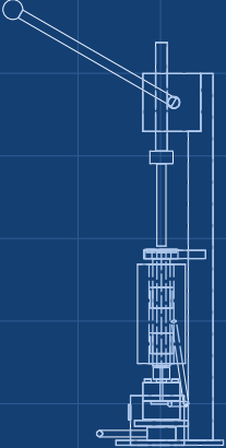
RIGHT VIEW Scale 1:20
