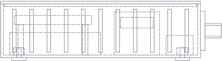
FRONT VIEW
