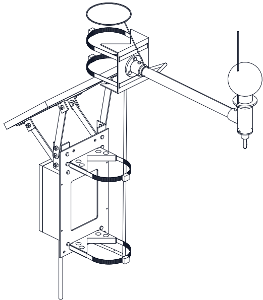
ISOMETRIC VIEW
