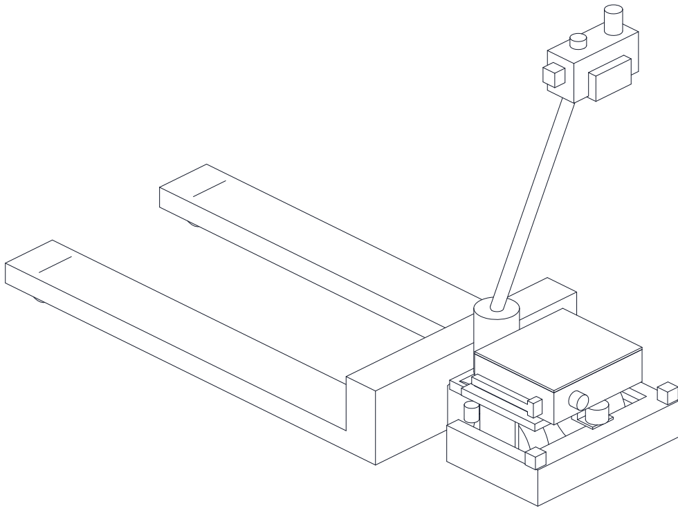
ISOMETRIC VIEW (DONOR JACK IS REFERENCE)
