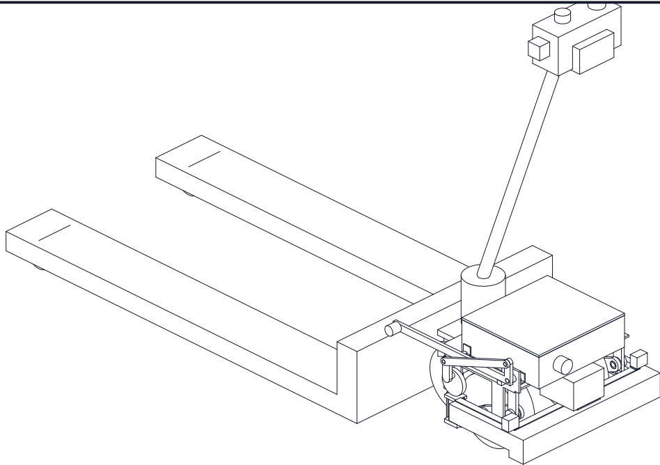
ISOMETRIC VIEW (DONOR JACK IS REFERENCE)
