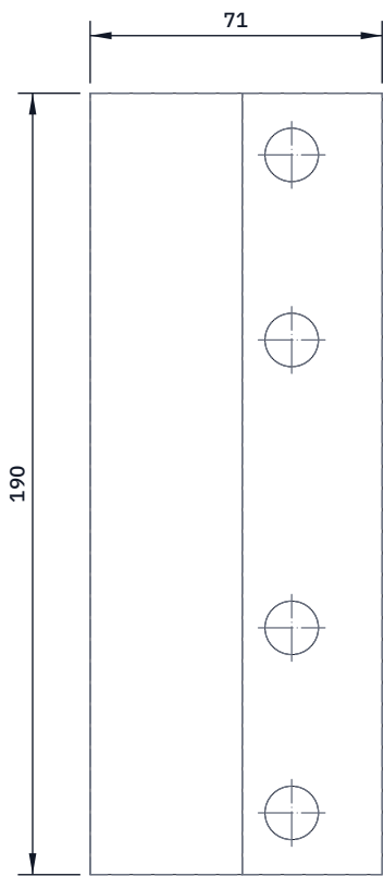
TOP VIEW Scale 1:2; looking down (along -Z)
