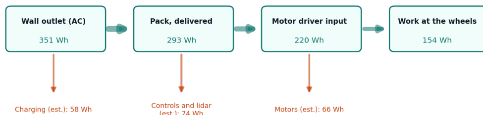
Figure 2. Energy per 8 h shift of 60 pallet moves, in Wh, from PLP-CAL-001. All values are estimates.
