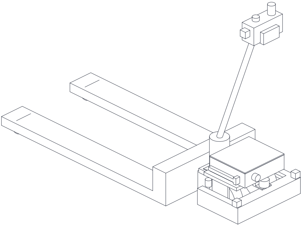
ISOMETRIC VIEW (DONOR JACK IS REFERENCE) Not to scale
