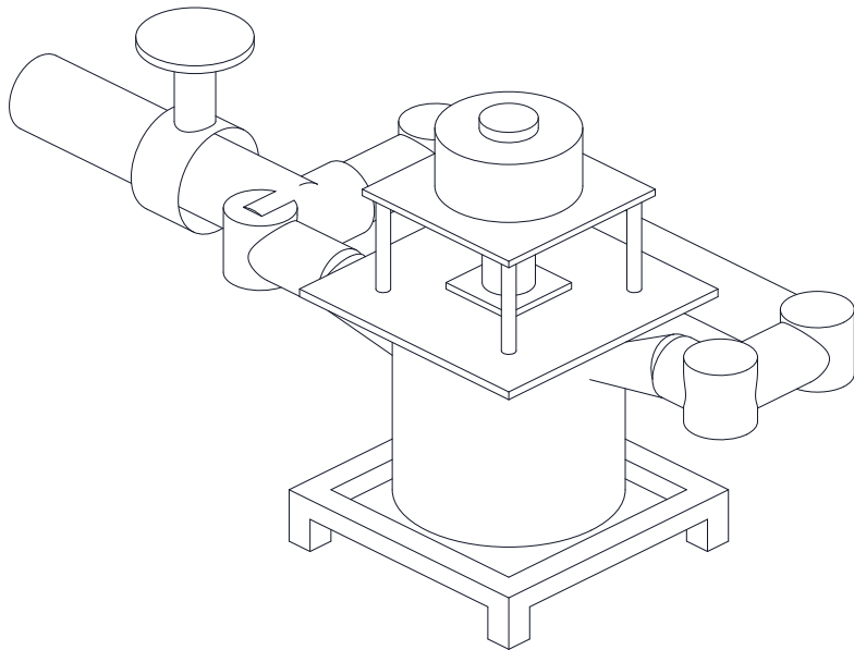
ISOMETRIC VIEW Not to scale; penstock shown as a stub
