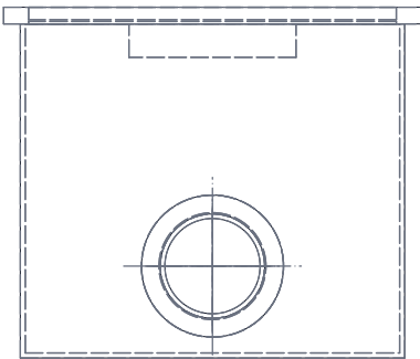
RIGHT VIEW Scale 1:10; looking at the right side (along -X)
