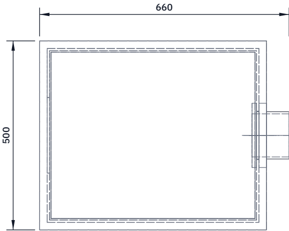
TOP VIEW Scale 1:10; looking down (along -Z)
