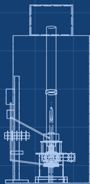
RIGHT VIEW
