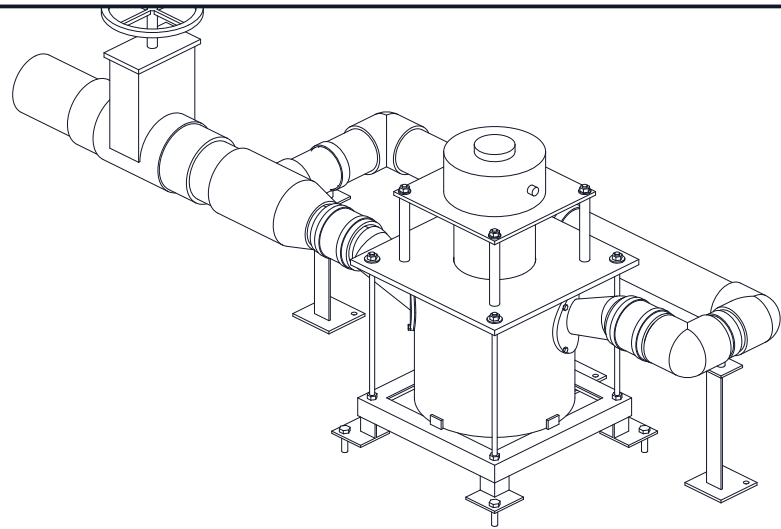
ISOMETRIC VIEW
