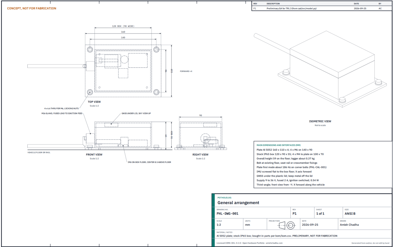
Figure 5. General arrangement PHL-DWG-001, Rev P1, generated from cad/src/model.py (PDF). Preliminary, not for fabrication.
