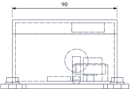
RIGHT VIEW
