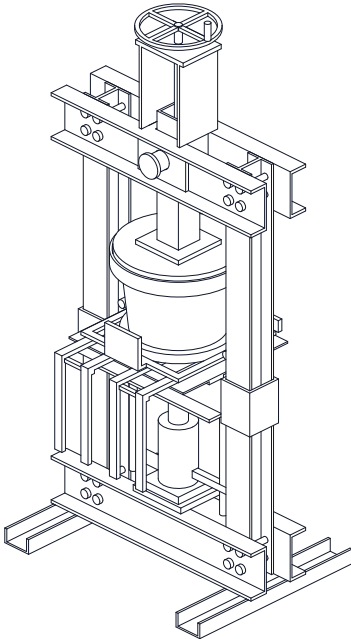
ISOMETRIC VIEW Not to scale; guards not shown
