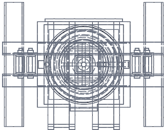
TOP VIEW Scale 1:20
