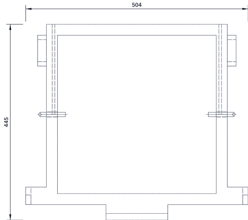
TOP VIEW
