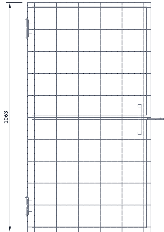
FRONT VIEW Scale 1:10; looking at the front (along +Y)
