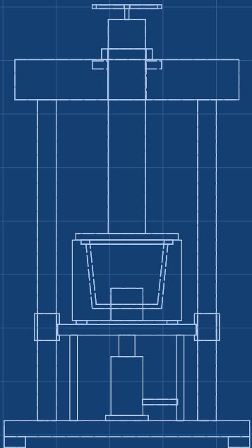
FRONT VIEW Scale 1:20
