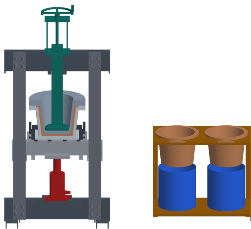
Front half removed, guards and gate left out; seen from the front and above, 18 deg elevation
