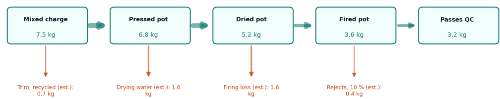
Figure 3. Material flow for one filter, from mixed charge to a filter that passes QC, in kg. All values are estimates from PPR-CAL-001.
