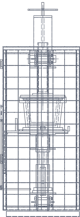
RIGHT VIEW
