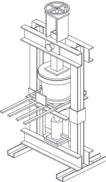
ISOMETRIC VIEW Not to scale; guards not shown
