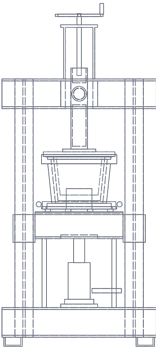
FRONT VIEW Scale 1:20
