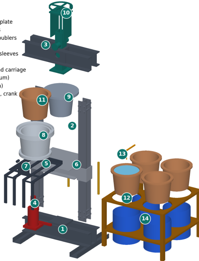
Figure 4. Exploded view with numbered callouts matching the BOM.
