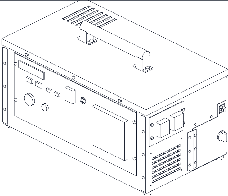
ISOMETRIC VIEW
