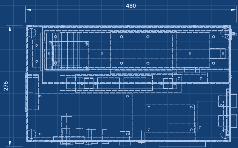
TOP VIEW Scale 1:5; looking down (along -Z)
