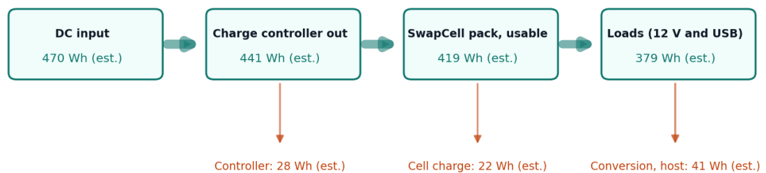
Figure 2. Energy per usable cycle, DC input to loads, from PBX-CAL-001. All values are estimates: controller 94 %, cell charge 95 %, output conversion for the reference evening mix of 12 V and USB loads.
