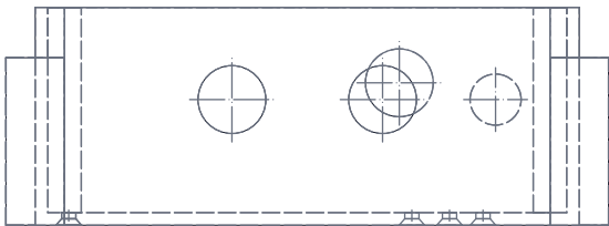
RIGHT VIEW
