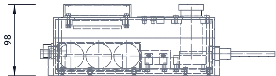
FRONT VIEW Scale 1:5; looking at the front (along +Y)
